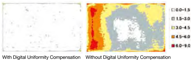
Color-separated image with Delta-E*ab distribution across the screen of the ColorEdge CG221 (gray level 128 measured)
